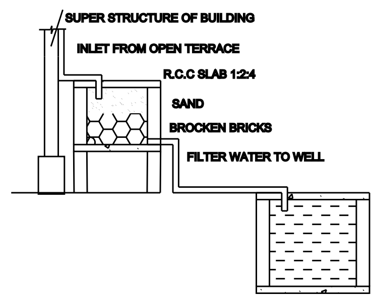
RAINWATER HARVESTING
