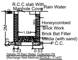
Details Of Rain Water Collection Pit (Recharge Well Method) SCALE: 1"=4'
