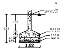
COLUMN FOUNDATION DETAILS
