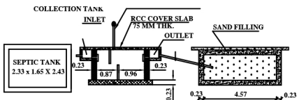
PLAN & SECTION ON SEPTIC TANK & DISP-TRENCH
