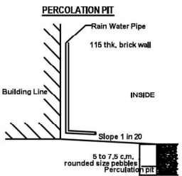
PERCOLATION PIT
