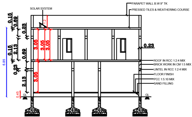
CROSS SECTION AB
