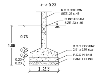
COLUMN FOUNDATION DETAILS
