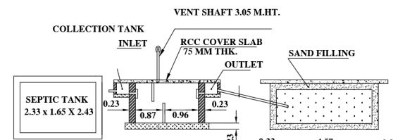
PLAN & SECTION ON SEPTIC TANK & DISP-TRENCH
