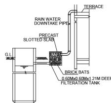
RAIN WATER HARVESTING SYSTEM
