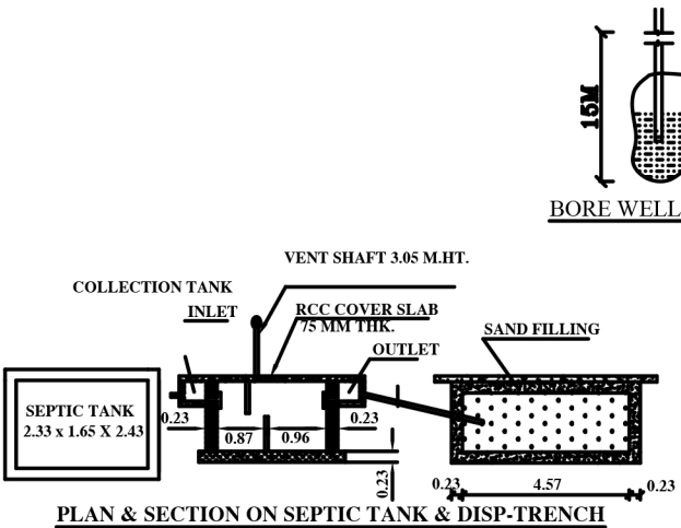
PLAN & SECTION ON SEPTIC TANK & DISP-TRENCH
