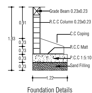
Foundation Details
