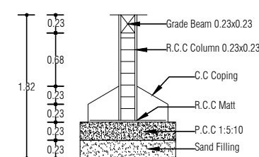
Foundation Detail
