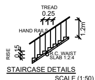
STAIRCASE DETAILS SCALE (1:50)
