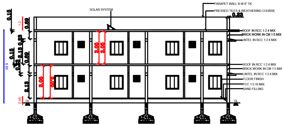
CROSS SECTION AB
