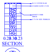
RAIN WATER HARVESTING 1.PERCOLATION PIT
