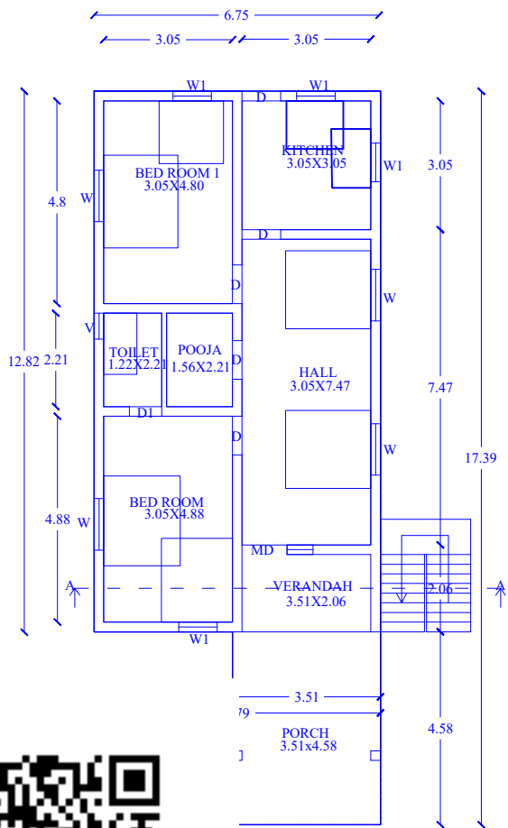
FLOOR PLAN
