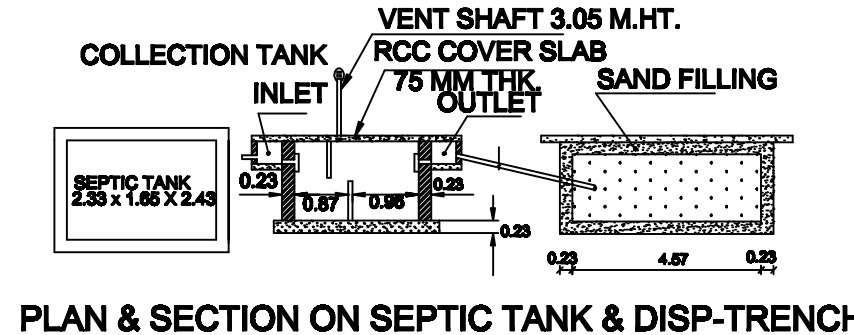
PLAN & SECTION ON SEPTIC TANK & DISP-TRENCH
