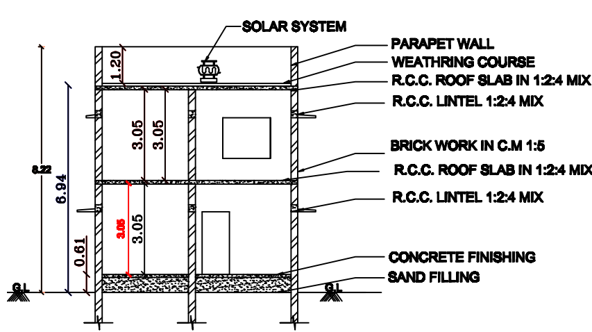
SECTION ON "AA,BB"
