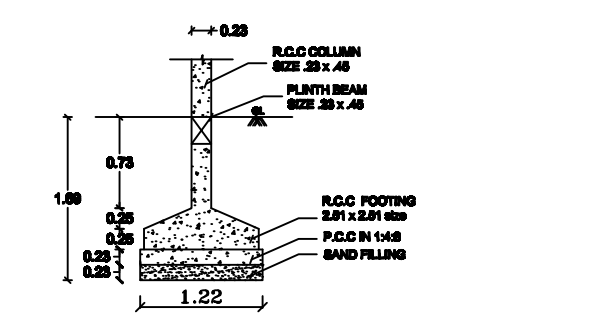
COLUMN FOUNDATION DETAILS
