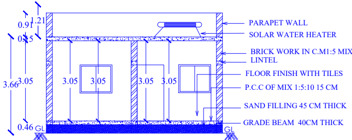
SECTION- AB
