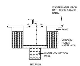
PLAN AND SECTION OF ORGANIC FILTRATIONS SUMP WITH COLLECTION WELL
