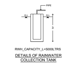
DETAILS OF RAINWATER COLLECTION TANK
