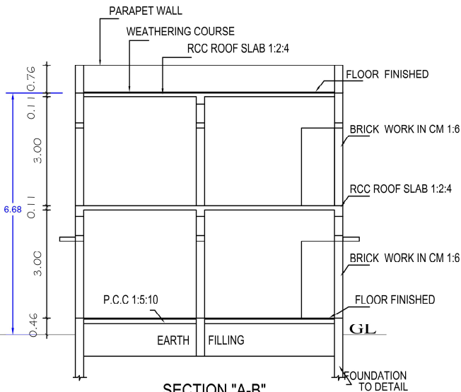
SECTION "A-B"
