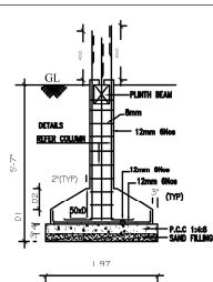
FOUNDATION DETAILS SCALE : 1:50.
