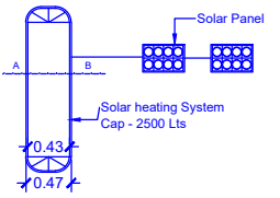
PLAN OF SOLAR WATER HEATING SYSTEM SCALE 1:50
