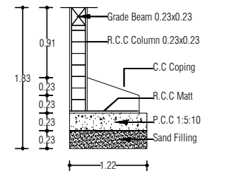
Foundation Details
