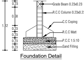
Foundation Detail
