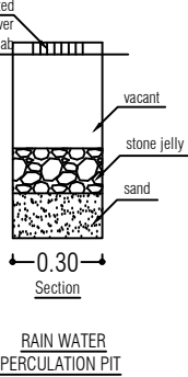
RAIN WATER PERCOLATION PIT
