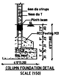
COLUMN FOUNDATION DETAILS SCALE (1/50)
