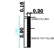
DETAILS OF PERCOLATION PIT RWVH_CAPACITY_L=1000 LTRS
