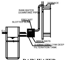
RAIN WATER HARVESTING SYSTEM
