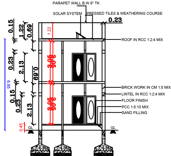
CROSS SECTION AB
