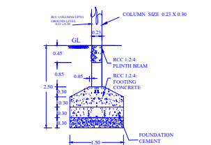
FOUNDATION DETAILS Scale: 1:50
