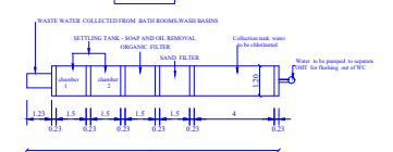
WASTE WATER RECYCLING SYSTEM
