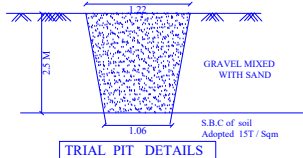
TRIAL PIT DETAILS
