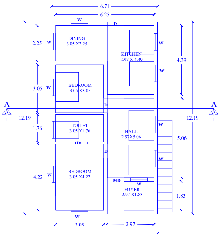
GROUND PLAN
