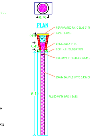
PERCOLATION PIT SECTION OF RAIN WATER RWH_CAPACITY_L=3.76
