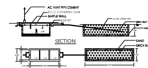
PLAN SEPTIC TANK AND TRENCH
