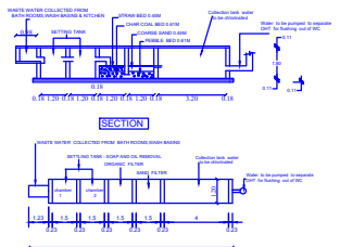
WASTE WATER RECYCLING SYSTEM
