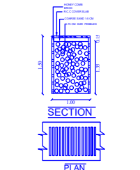
RAIN WATER HARVESTING PERCOLATION BED
