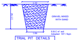
TRIAL PIT DETAILS
