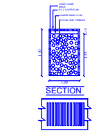
SECTION RAIN WATER HARVESTING PERCOLATION BED
