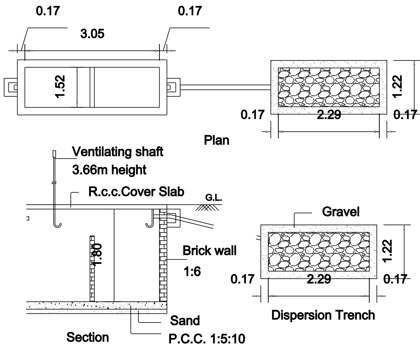
Details of Septic Tank
