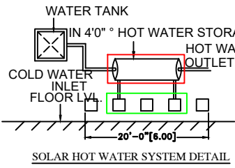
SOLAR HOT WATER SYSTEM DETAIL
