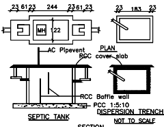
SEPTIC TANK
