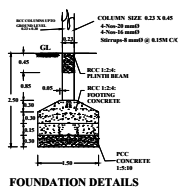
FOUNDATION DETAILS
