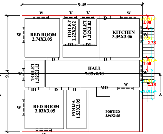
EXISTING GROUND FLOOR PLAN
