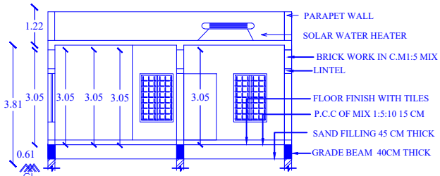
SECTION ON A-A1
