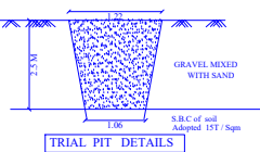
TRIAL PIT DETAILS
