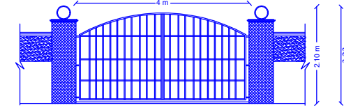
COMPOUND GATE (NOT TO SCALE)
