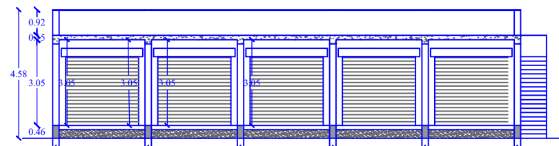
SECTION ON A-A
