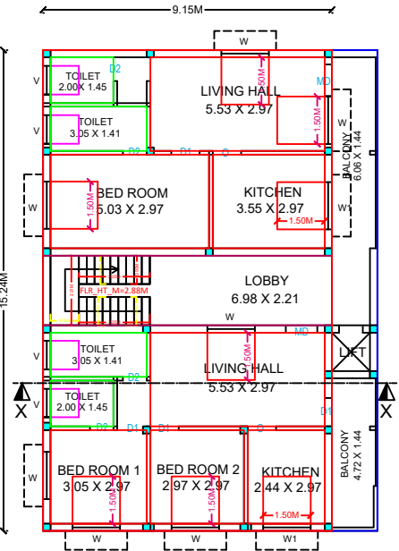
PRO. SECOND FLOOR PLAN
