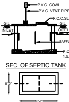
PLAN OF SEPTIC TANK
