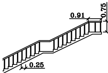
STAIRCASE SECTION
