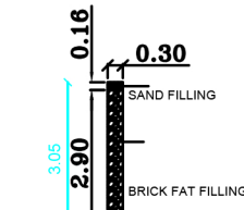
DETAILS OF PERCOLATION PIT RWH_CAPACITY_L=1000 LTRS
