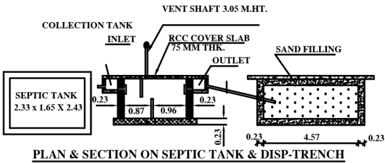
PLAN & SECTION ON SEPTIC TANK & DISP-TRENCH
