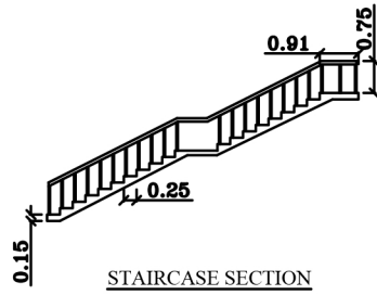
STAIRCASE SECTION
