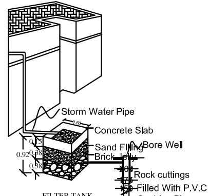
RAIN WATER STORAGE ARRANGEMENTS
