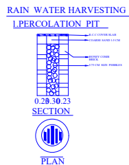
RAIN WATER HARVESTING PERCOLATION PIT
