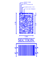
RAIN WATER HARVESTING PERCOLATION BED
