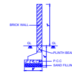
COMPOUND WALL DETAIL
