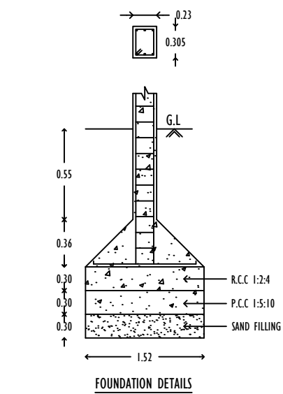
FOUNDATION DETAILS
