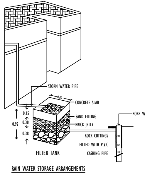
RAIN WATER STORAGE ARRANGEMENTS
