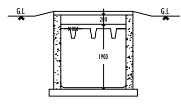
SECTIONAL ELEVATION - BB
