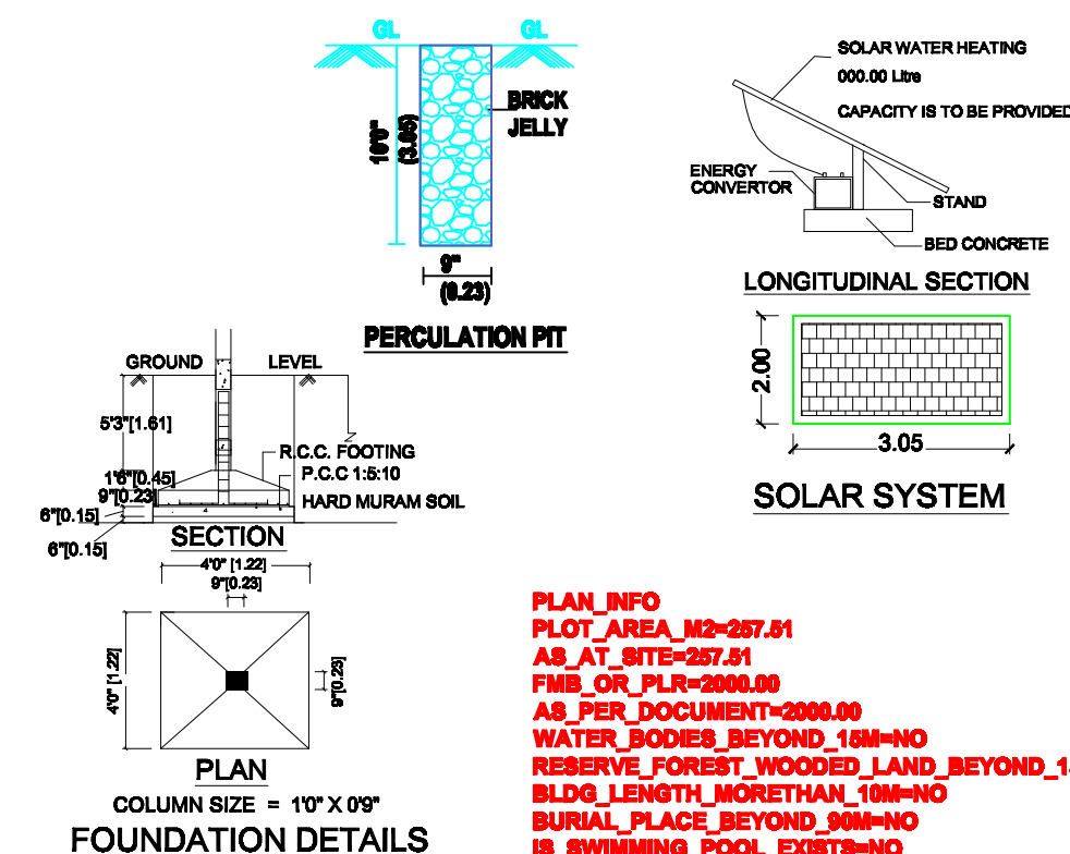
FOUNDATION DETAILS
