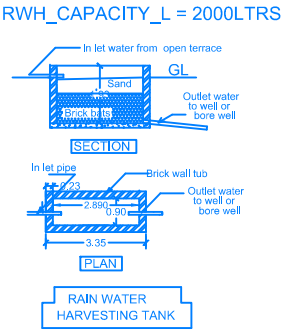
RWH_CAPACITY_L = 2000LTRS
