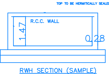
RWH_SECTION (SAMPLE)
