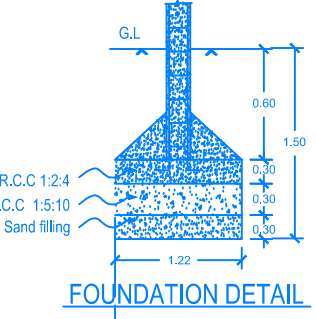
FOUNDATION DETAIL
