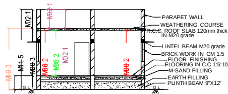
SECTION ON XX
