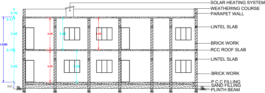
SECTION ON-'AA'
