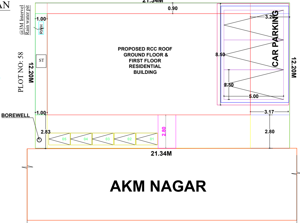
SITE PLAN (1:100)
