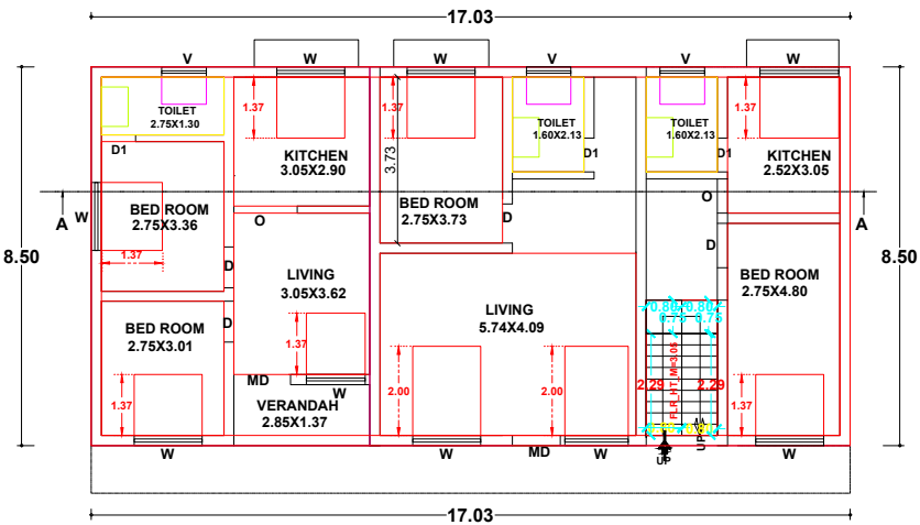
PRO.FIRST FLOOR PLAN
