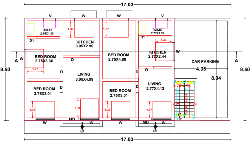
PRO.GROUND FLOOR PLAN
