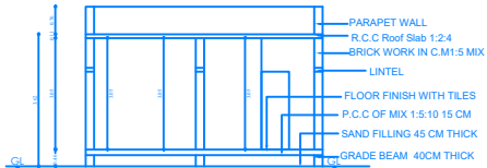
SECTION ON - AA
