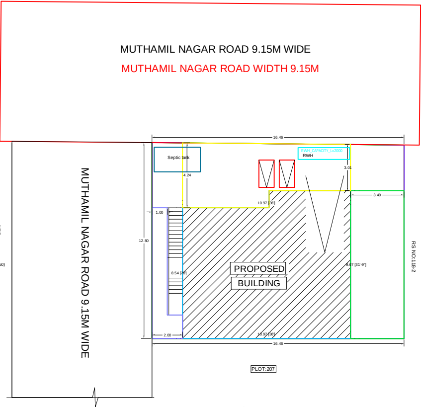
SITE PLAN
