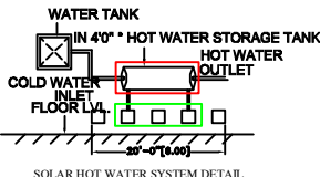
SOLAR HOT WATER SYSTEM DETAIL
