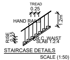
STAIRCASE DETAILS SCALE (1:50)
