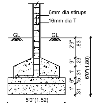
COLUMN FOUNDATION DETAIL SCALE (1:50)
