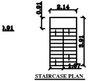
STAIRCASE PLAN
