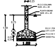
COLUMN FOUNDATION DETAILS
