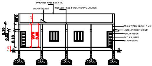
CROSS SECTION AB
