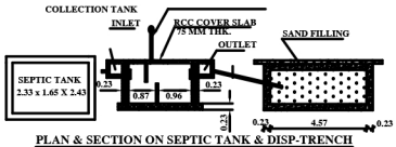
PLAN & SECTION ON SEPTIC TANK & DISP-TRENCH
