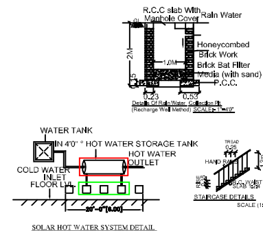
SOLAR HOT WATER SYSTEM DETAIL
