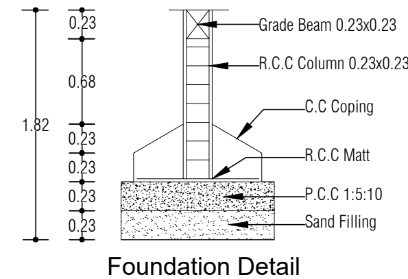
Foundation Detail
