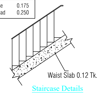
Staircase Details
