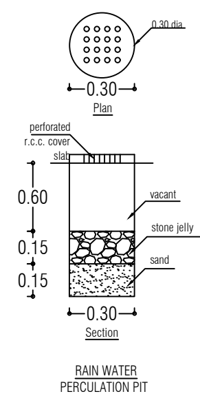
RAIN WATER PERCOLATION PIT
