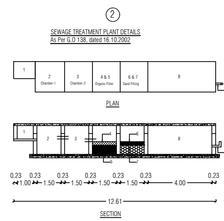
WASTE WATER RECYCLING SYSTEM:
