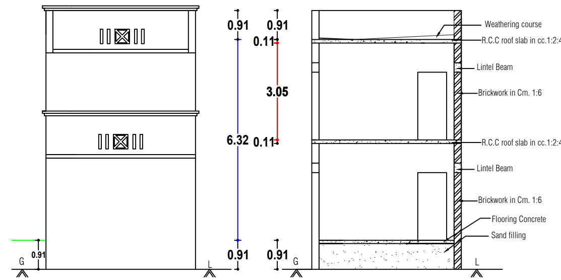
FRONT ELEVATION
