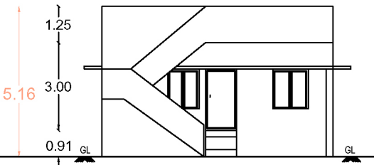
FRONT ELEVATION
