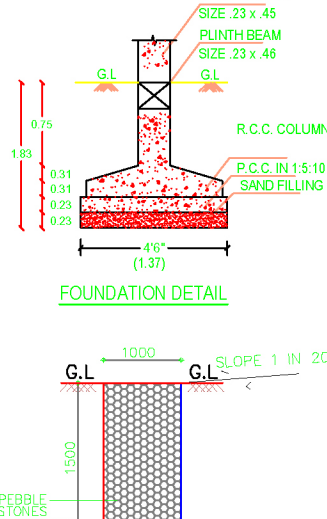
FOUNDATION DETAIL SCALE : 1: = 100
