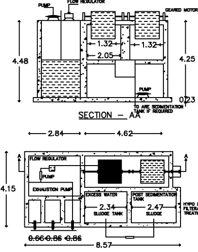
SEWAGE TREATMENT PLANT [S.T.P] WASTER WATER FILTERATION BY RECIRCULATION SYSTEM G.O(MS) NO.138 D.T.11-10-02 SCALE : 1:100
