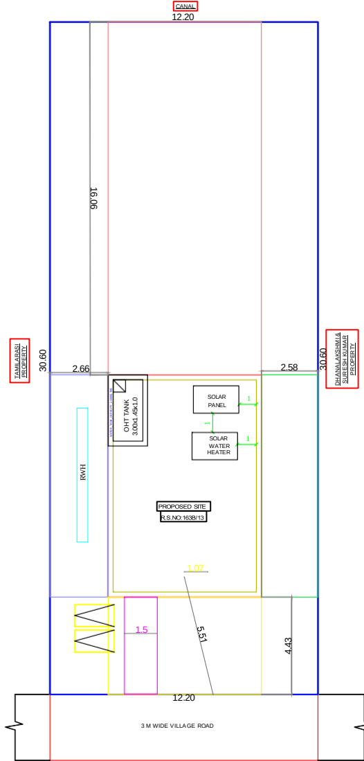
SITE PLAN SCALE IN ~ 1:100
