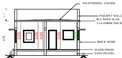
SECTION ON "XX"
