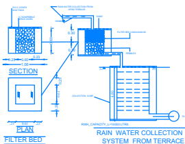
RAIN WATER COLLECTION SYSTEM FROM TERRACE
